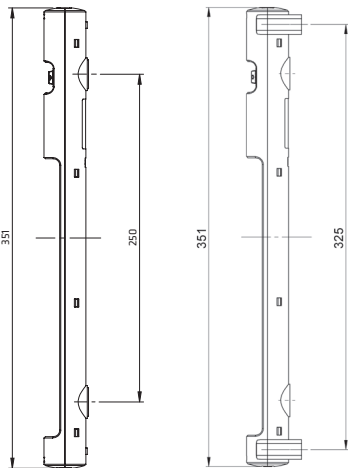
LED 025 multi wide voltage with magnet or screw fixing
